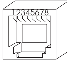
Figure 5 — Modular Jack Numbering Orientation
