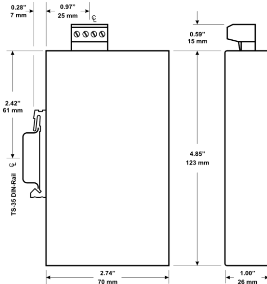
Figure 5 — Product Dimensions
